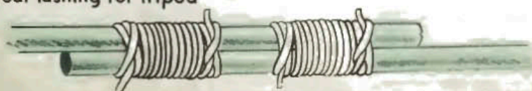
Shear lashings for extending poles
